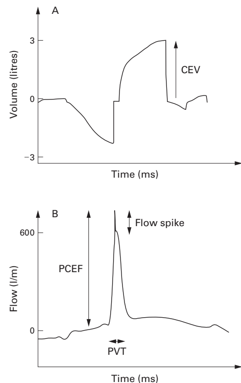
Figure 1 Normal recordings of (A) cough expiratory volume (CEV) and (B) cough expiratory flow. The peak cough expiratory flow rate (PCEF) was measured from the initiation of a positive flow rate to the maximum obtained value. This included the flow spike if present. The peak value time (PVT) was measured as the time taken from initiation of a positive flow rate to the PCEF. The cough expiratory flow volume was taken as the maximum expiratory volume recorded.
